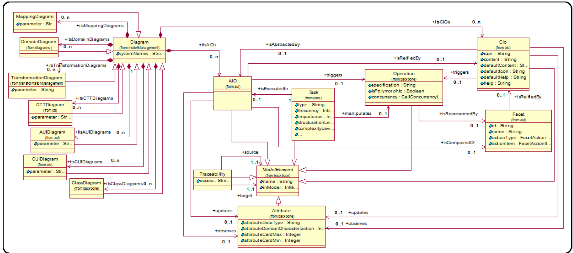
Figura A.9: Package Mapping
