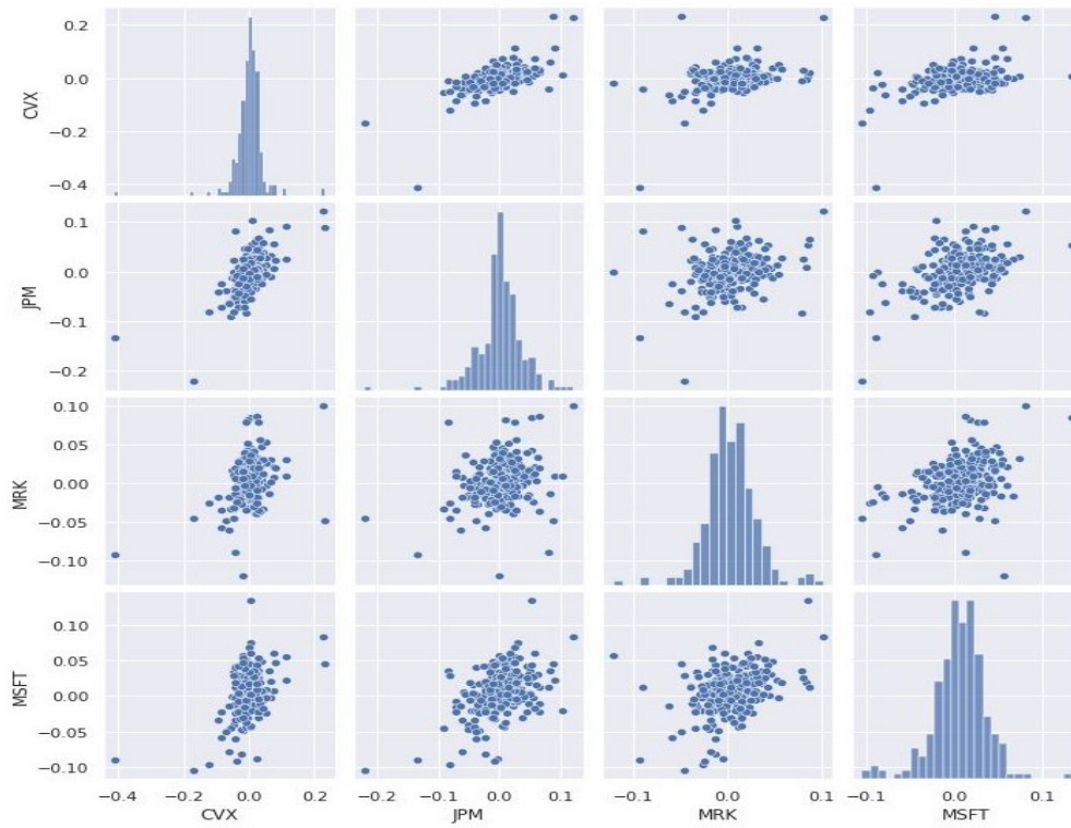
Figure 13: Distribution
