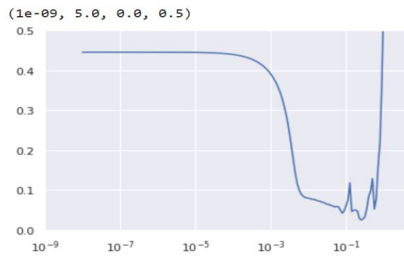
Figure 15: Tuning Learning Rate
