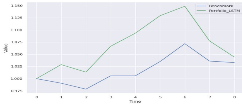
Figure 20: May 20 - Jun 20
