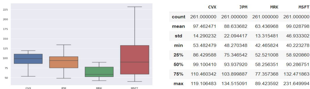
Figure 4: Return Boxplot
