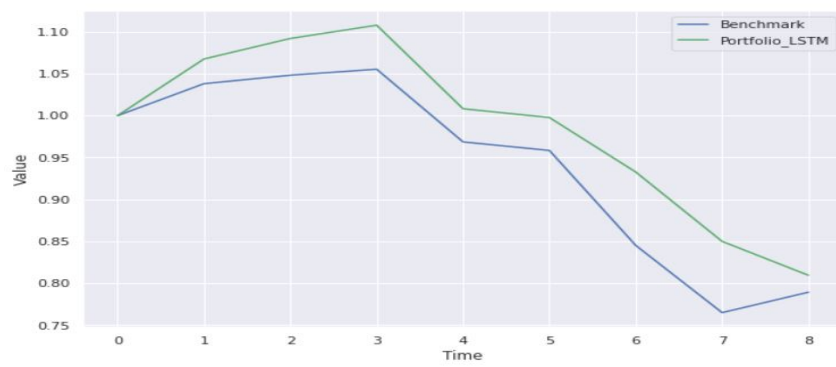
Figure 19: Feb 20 - Mar 20
