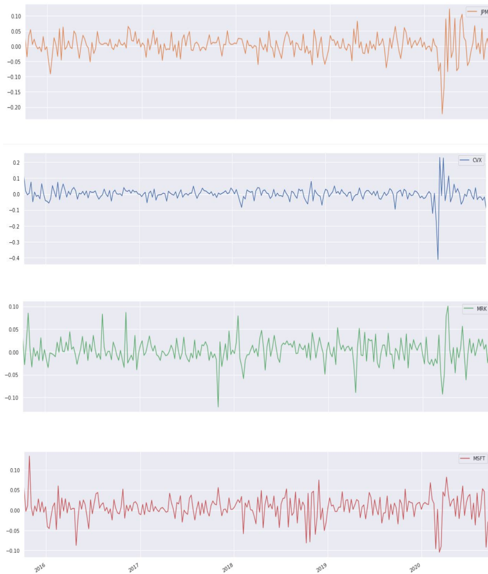
Figure 11: Stock's Return
