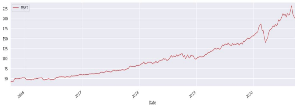
Figure 1: Stock's Prices
