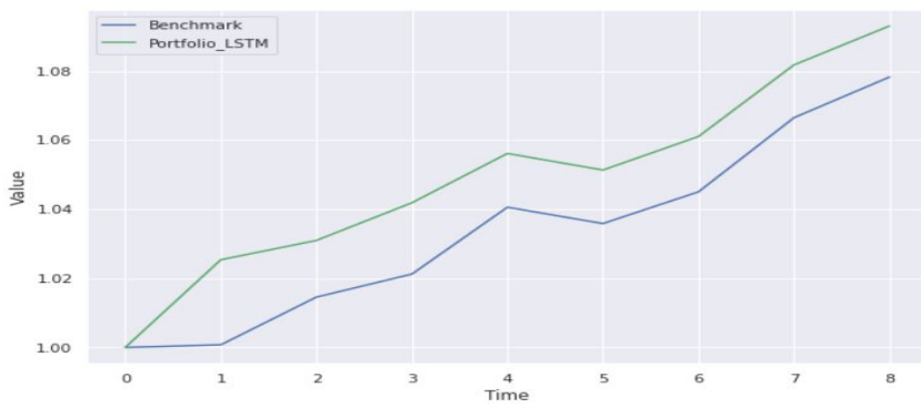
Figure 18: Nov 19 - Dic 19
