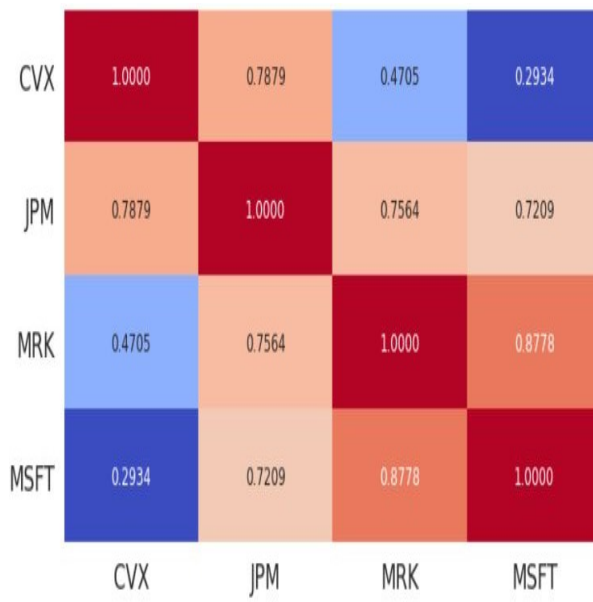
Figure 12: Correlation
