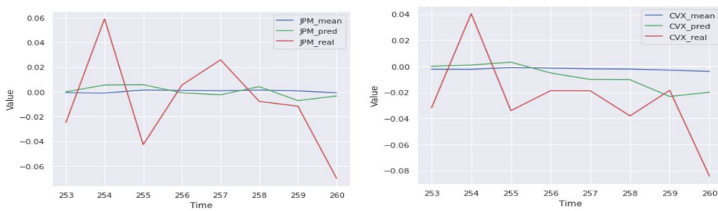
Figure 6: Stock’s Return
