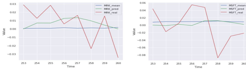
Figure 7: Stock's Return
