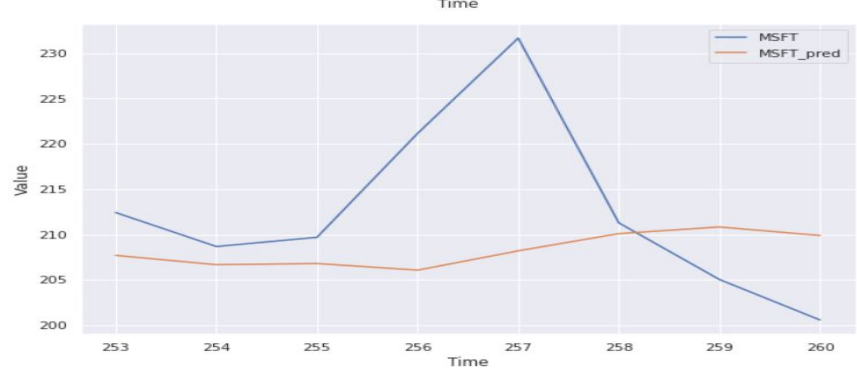
Figure 16: Stock's Prices
