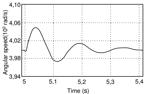
(c) Estimated angular speed under load torque
