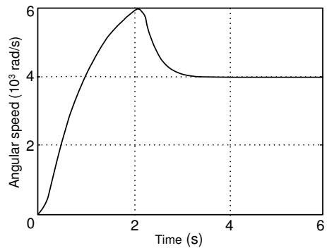
(b) Estimated angular speed
