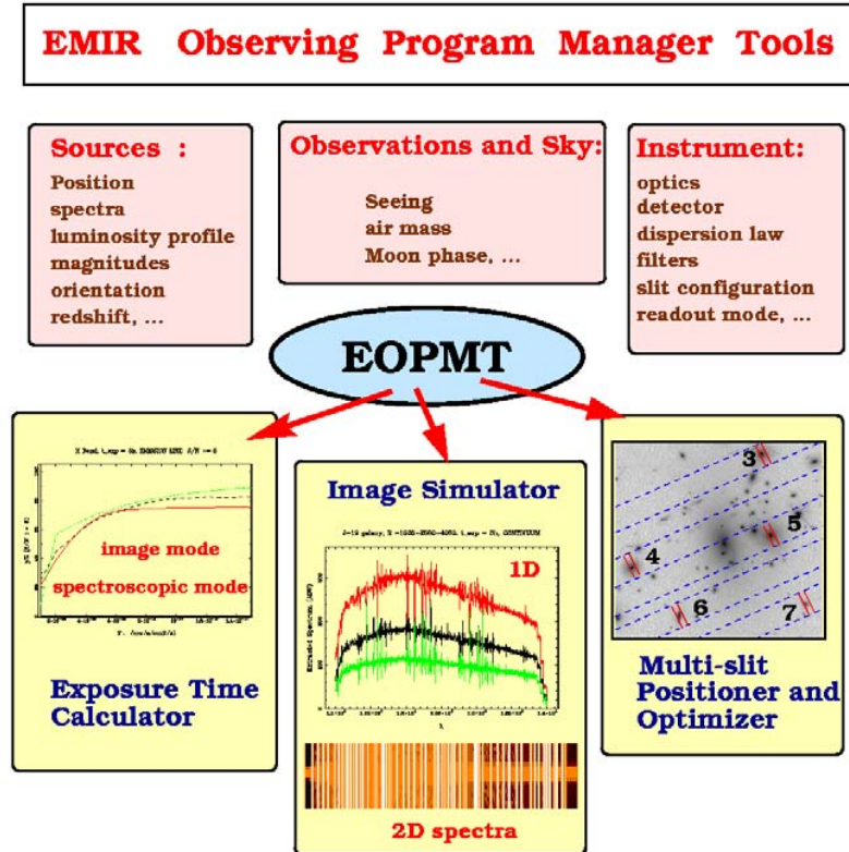
Fig. 7. Schematic view of the EOPMS.
