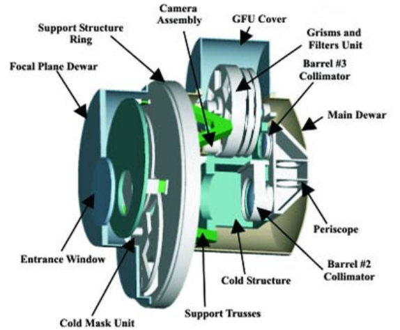
Fig. 5. EMIR mechanical layout, with the wheel for the slit masks.
