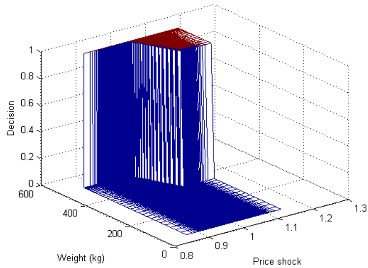
Fig. 6 Policy function
