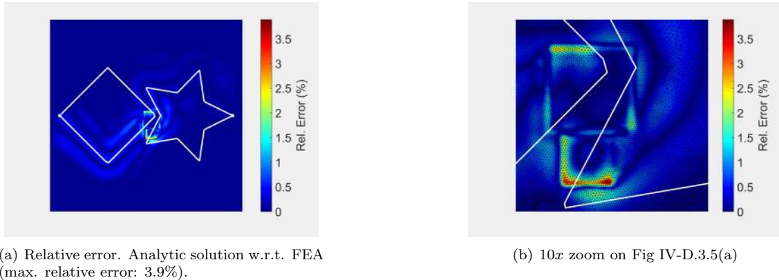
Figure IV-D.3.5: Appraisal of our analytic solution (Fig IV-D.3.3(d)) vs the FEA solution (Fig IV-D.3.4(c))
