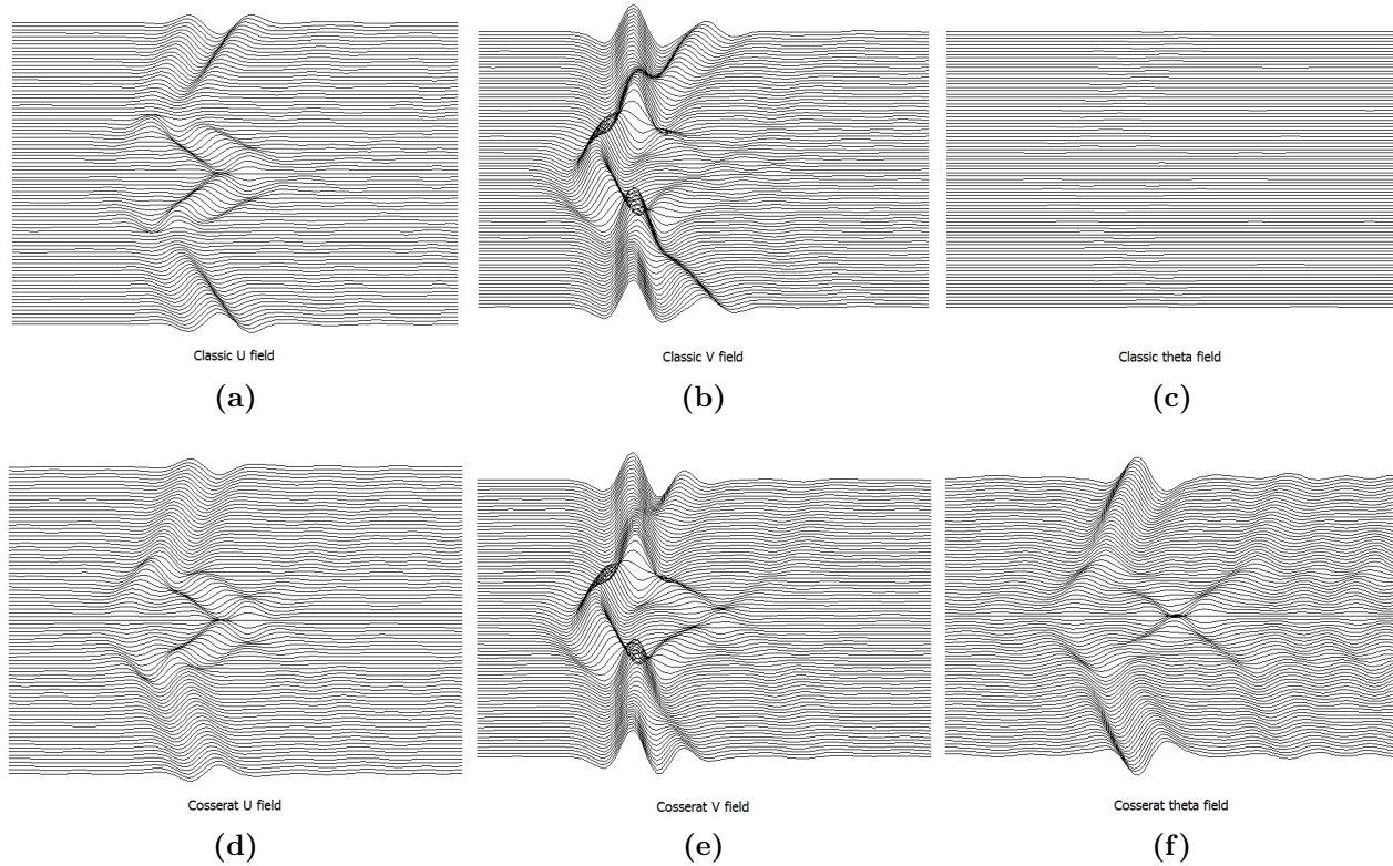
Figure 4.3. Synthetic seismograms for the semi-circular canyon in a micropolar half-space under vertically incident P waves.
